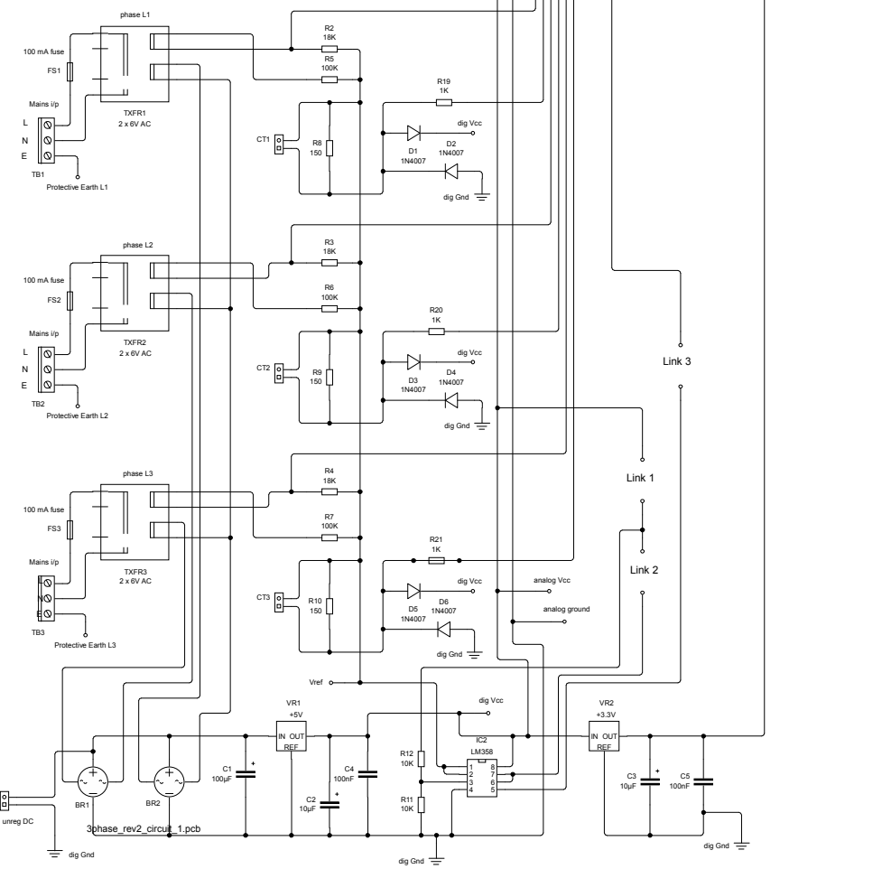
Circuit diagram for Mk2 PV Router, 3-phase, rev 2 Robin Emley, October 2015 www.mk2pvrouter.co.uk
